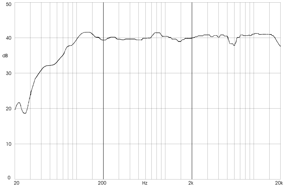
Fig 1. On axis anechoic frequency response
